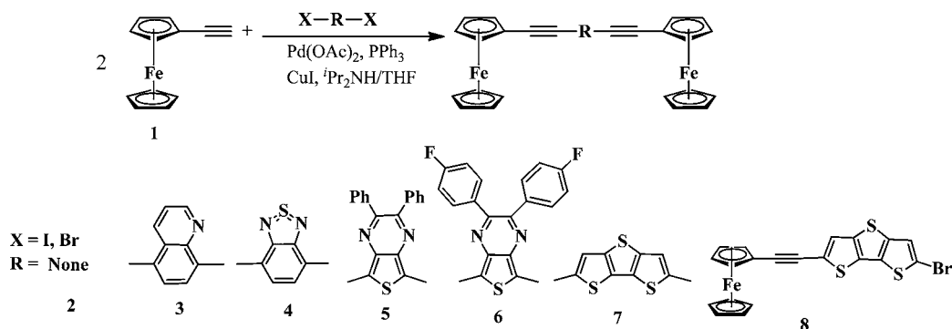
Scheme 1. Synthesis of Bis(ferrocenylethynyl) Complexes 2–7 and Mono(ferrocenylethynyl) Complex 8
