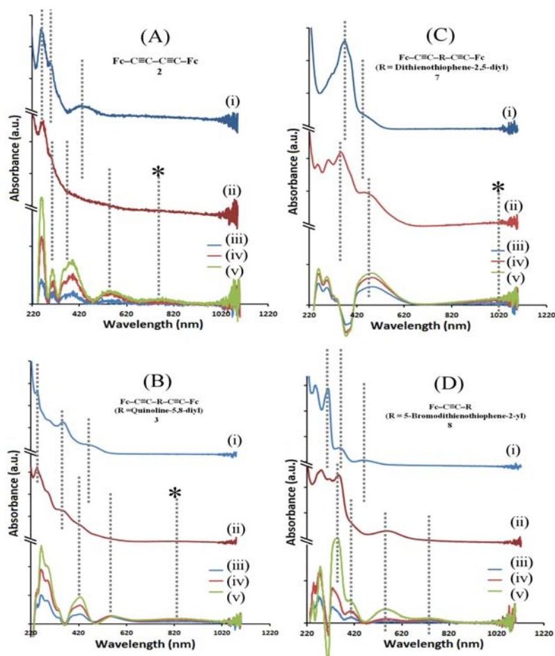
Figure 6. UV-vis spectra of complexes 2 , 3 , 7 , and 8 in a DCE solution at different potentials applied in OTTLE cells with [n\text{-Bu}_4\text{N}]\text{PF}_6 as the supporting electrolyte [data for the neutral spectra (i), the monocation (ii), and difference spectra (iii–v) are shown]: (A) 2 with (i) neutral, (ii) 650 mV, and (iii–v) 540, 650, and 710 mV; (B) 3 with (i) neutral, (ii) 620 mV, and (iii–v) 580, 620, and 660 mV; (C) 7 with (i) neutral, (ii) 630 mV, and (iii–v) 600, 630, and 660 mV; (D) 8 with (i) neutral, (ii) 650 mV, and (iii–v) 620, 650, and 690 mV, respectively.
